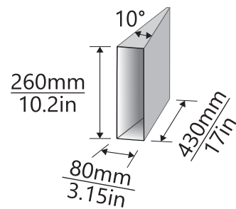
TYPE B2
